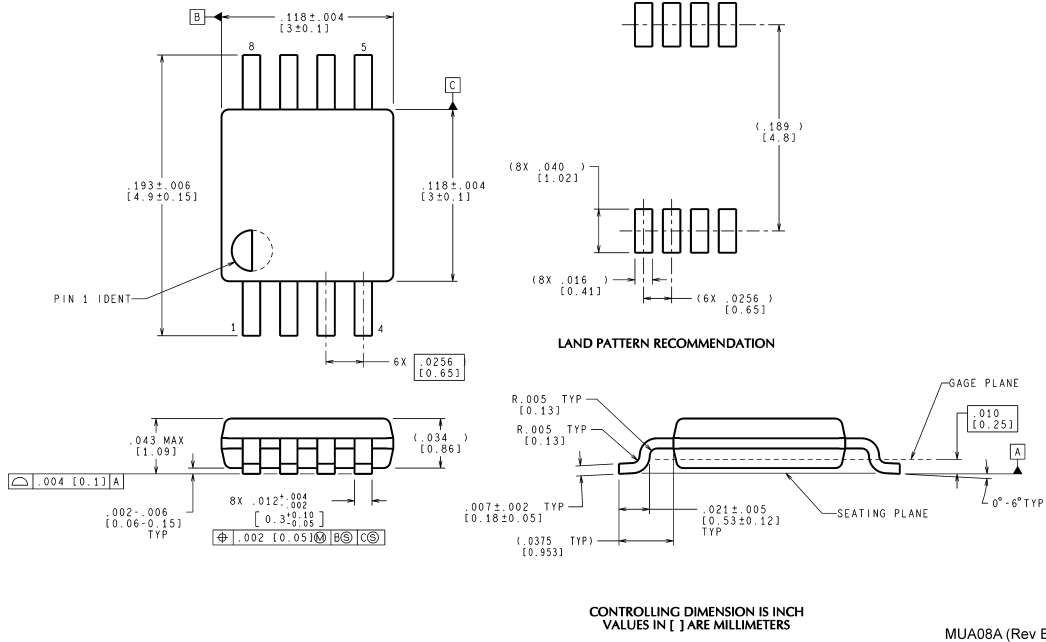
8-Pin MSOPNS Package Number MUA08A
