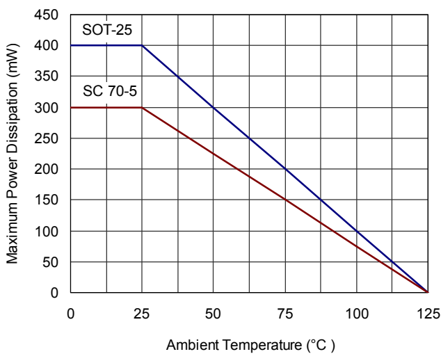
Figure 2. Derating Curve for Packages
