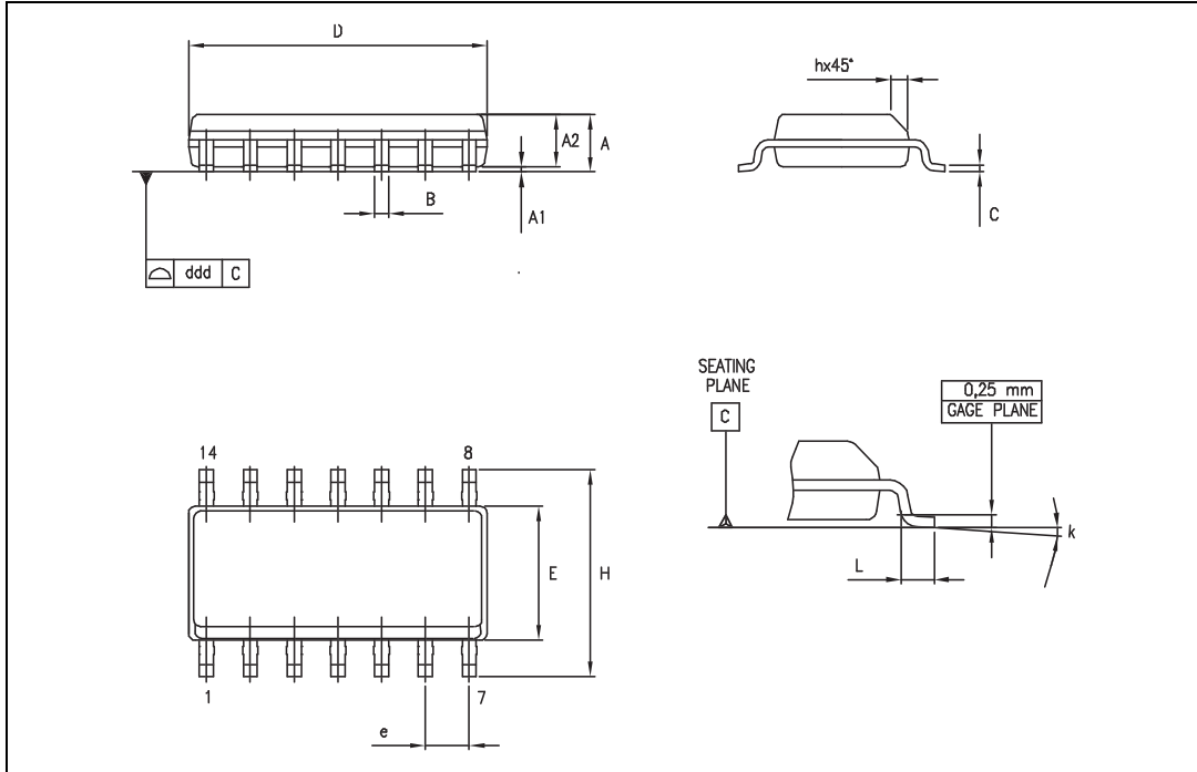
Figure 16. SO-14 package mechanical drawing
