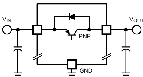
Figure 22. Reverse Current Path
