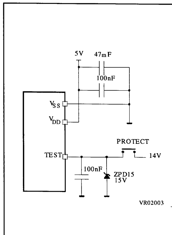
Figure 34. Programming Circuit
