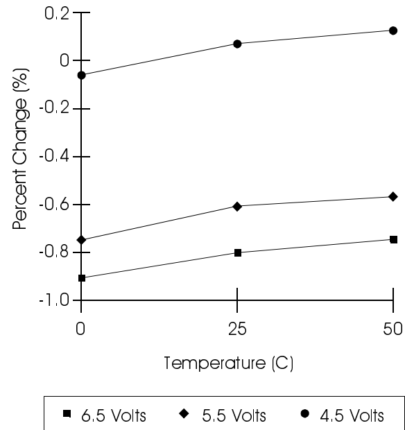
Chart 8: Oscillator Stability
