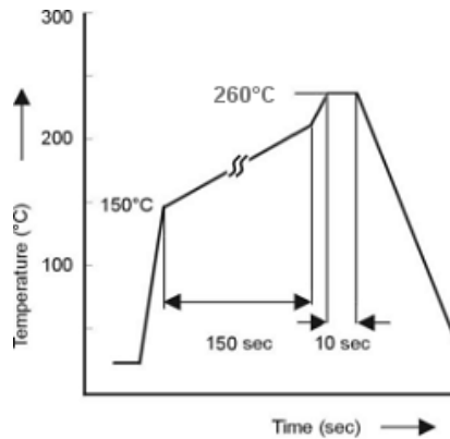
soldering condition
