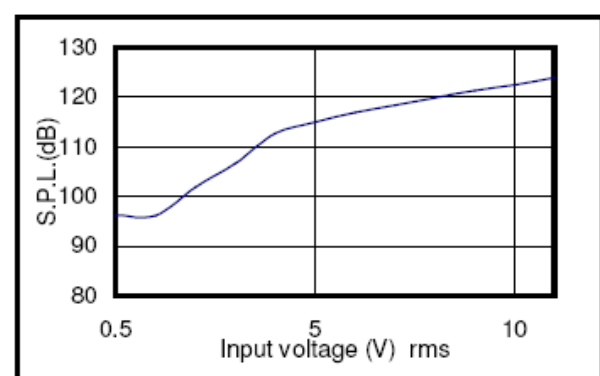
S.P.L. change with driving voltage
