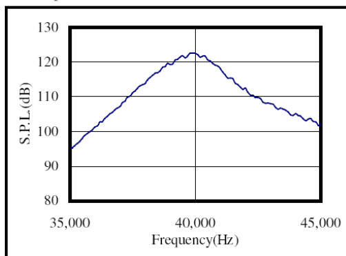
Sound pressure level
